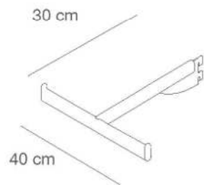
3BAP2 Barra appenderia piccola finitura cromo opaco Straight frontal crossbar matt chromium finishing L.40 x P. 30 cm
