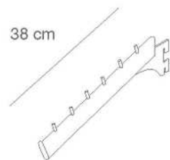
3APFZ Appenderia frontale inclinata finitura cromo opaco Tilted frontal crossbar matt chromium finishing L.38 cm
